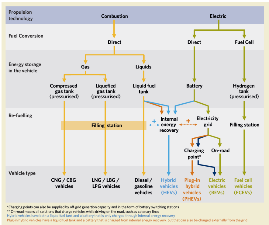
Figure 9 Vehicle technologies for road transport, (REN21, 2021)
