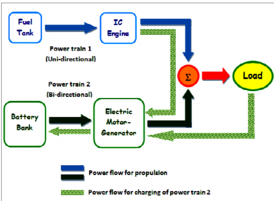
Figure 7 Retrofitting of existing vehicle into hybrid vehicle, (Saiful Zulkifli, 2012)
